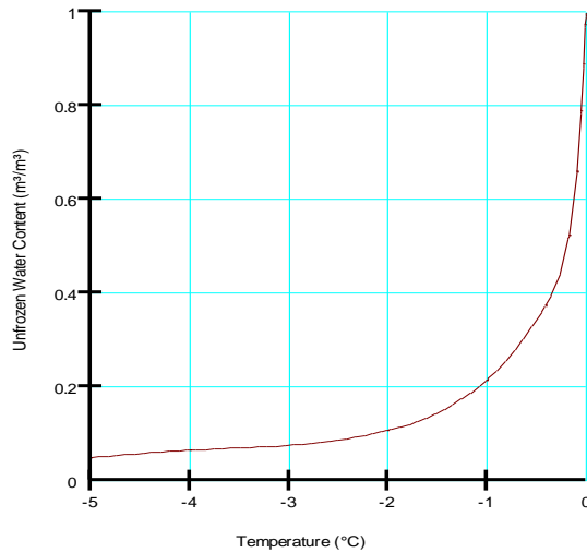
Figure 3. Example of an unfrozen water content versus temperature function.
