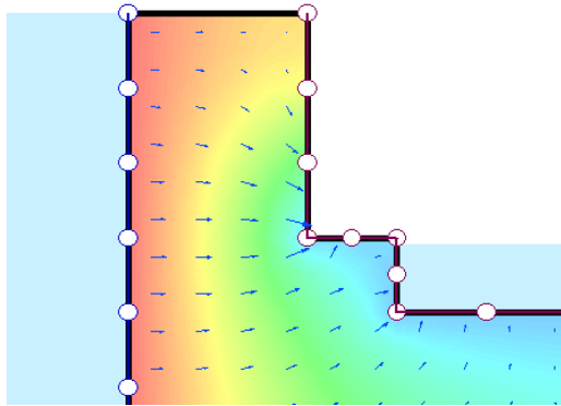
Figure 2. Example of the Total Head versus Volume boundary condition applied to the inside of an excavation.
