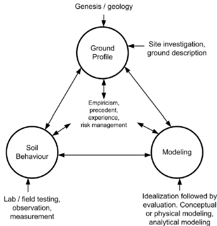
Figure 8. Burland Triangle (Ground Engineering, 1996).
