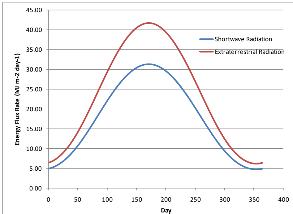
Figure 4. Estimated extraterrestrial and shortwave radiation at Latitude 52.17 degrees ( a_s = 0.25 ; b_s = 0.5 ).
